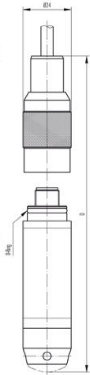
Fig. 4: Electrical connection, connectable
